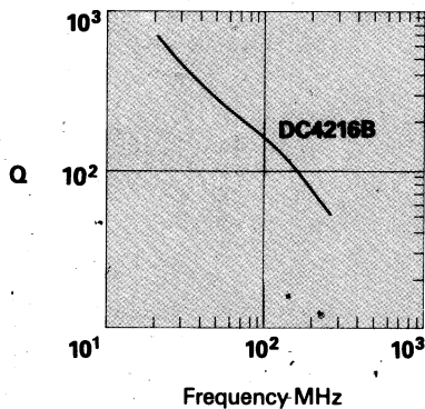
TYPICAL Q vs. FREQUENCY
