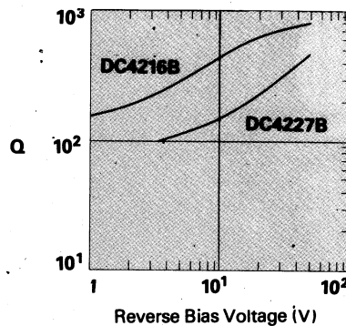
TYPICAL Q vs. REVERSE BIAS VOLTAGE
