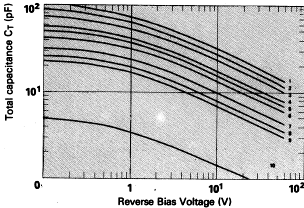
TYPICAL CAPACITANCE vs. TUNING VOLTAGE
