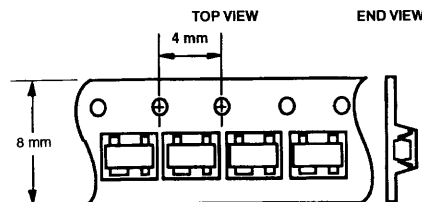
Figure 5. Option L31 for SOT-143 Packages.
