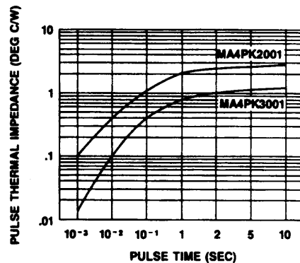
PULSED THERMAL IMPEDANCE
