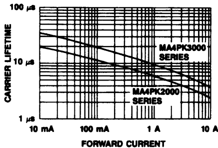
CARRIER LIFETIME vs FORWARD CURRENT
