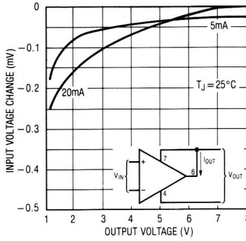
Shunt Gain
