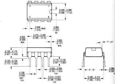
N8 Package 8 Lead Plastic
