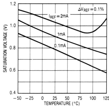
Output Saturation
