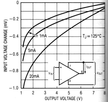
Shunt Gain
