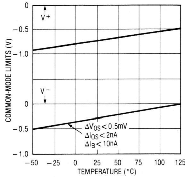
Common-Mode Limits
