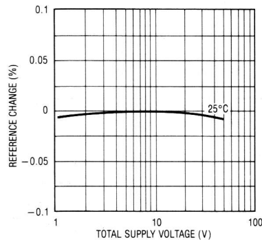
Line Regulation
