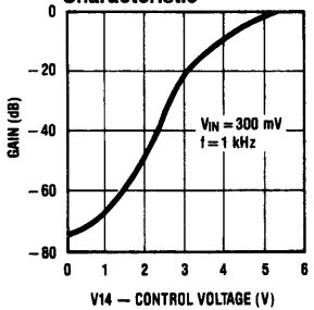
Volume Control Characteristic
