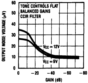
Output Noise Voltage vs Gain
