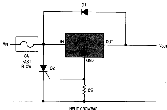
INPUT CROWBAR
