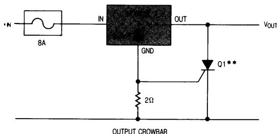
OUTPUT CROWBAR
