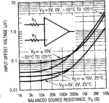
Offset Voltage vs Balanced Source Resistor
