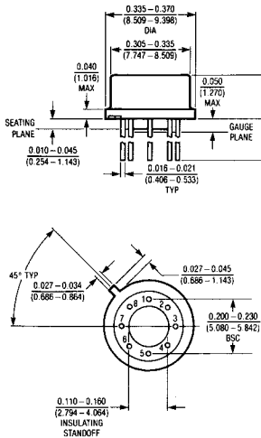
H8 Package TO-5 Metal Can
