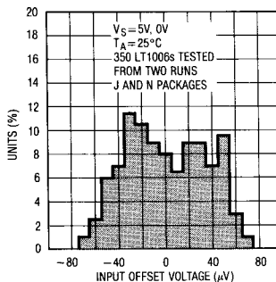
Distribution of Input Offset Voltage
