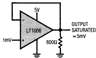
Voltage Follower
