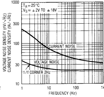
Noise Spectrum
