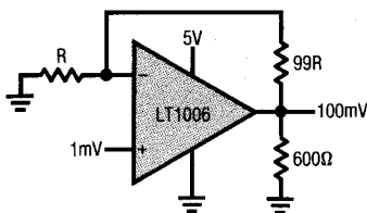
Gain 100 Amplifier
