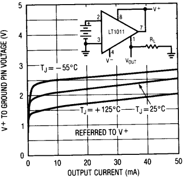
Output Saturation— Ground Output
