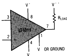
Driving Load Referenced to Positive Supply
