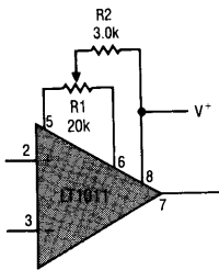
Offset Balancing
