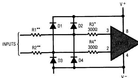
Limiting Fault Input Currents
