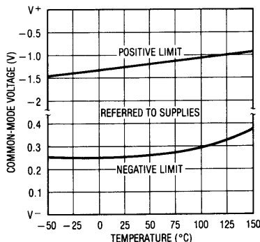
Common-Mode Limits
