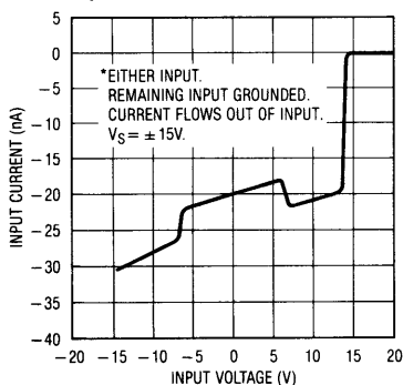
Input Characteristics*
