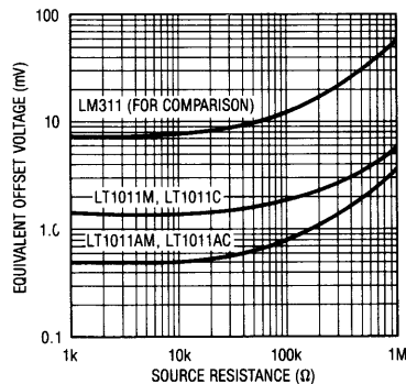
Worst-Case Offset Error
