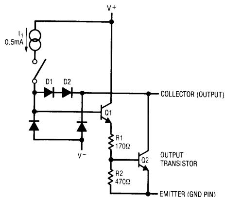
Output Transistor Circuitry
