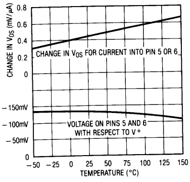
Offset Pin Characteristics
