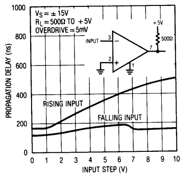
Response Time vs Input Step Size
