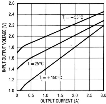
Minimum Input-Output Differential of Main Output
