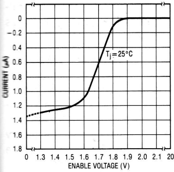
Enable Pin Characteristics
