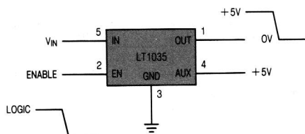
Functional Diagram
