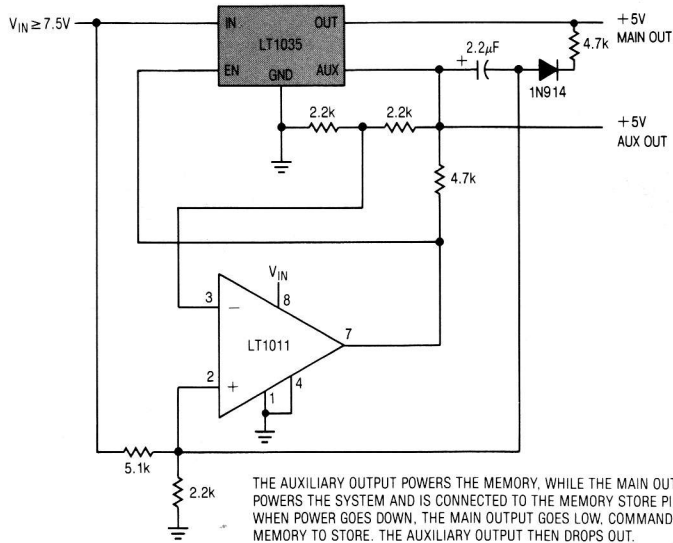
Line Dropout Detector
