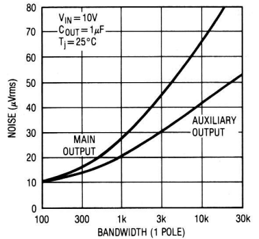
Output Noise
