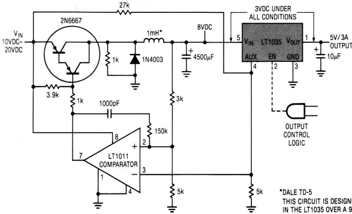
Low Dissipation Regulator
