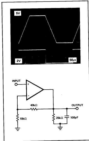
NONINVERTING LARGE-SIGNAL RESPONSE
