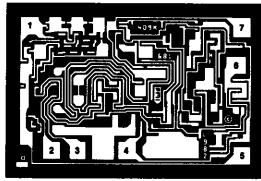
DIE SIZE 0.069 × 0.046 inch, 3174 sq. mils (1.75 × 1.17 mm, 2.05 sq. mm)
