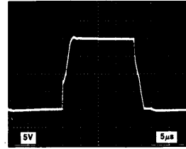
FIGURE 8: Follower Feedforward Transient Response
