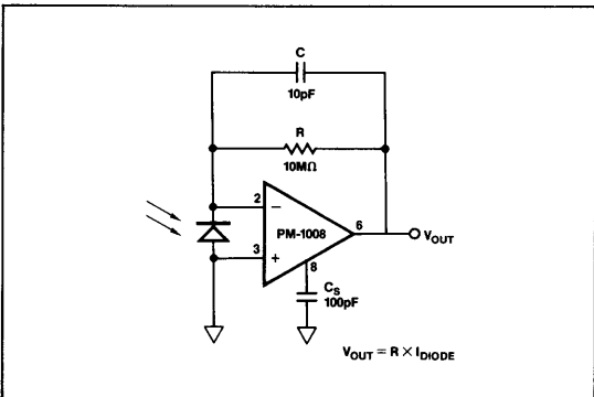
FIGURE 11: Photodiode Amplifier
