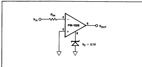
FIGURE 12: Zero-Crossing Detector
