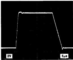
FIGURE 7: Follower Feedforward Compensation
