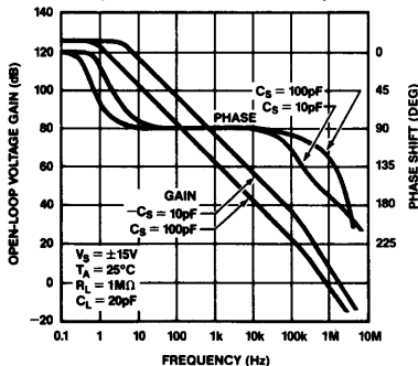
OPEN-LOOP GAIN, PHASE vs FREQUENCY (ALT. COMPENSATION)
