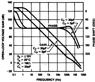
OPEN-LOOP GAIN, PHASE vs FREQUENCY (STD. COMPENSATION)
