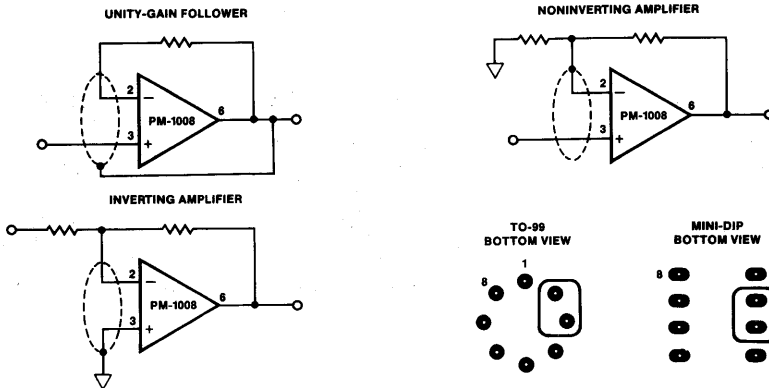
FIGURE 9: Guard Ring Layout and Connections
