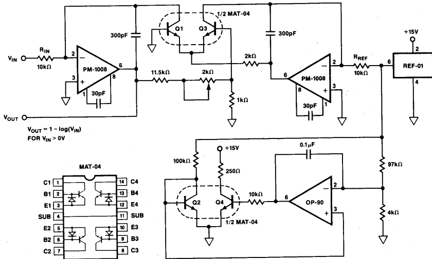
FIGURE 13: Logarithmic Amplifier with Heated Logging Transistors
