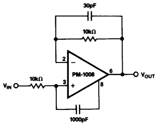
FIGURE 7: Follower Feedforward Compensation
