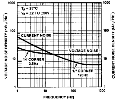
NOISE DENSITY vs FREQUENCY
