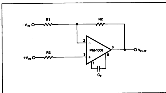
FIGURE 1: Standard Frequency Compensation
