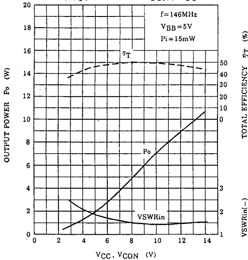
Po, \eta_T , VSWRin - VCON, VCC
