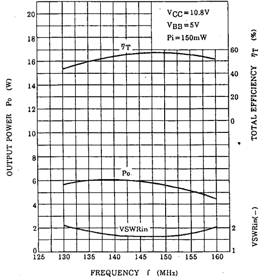
Po, \eta_T , VSWRin - f
