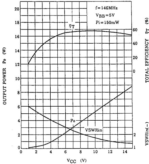
Po, \eta_T , VSWRin - VCC
