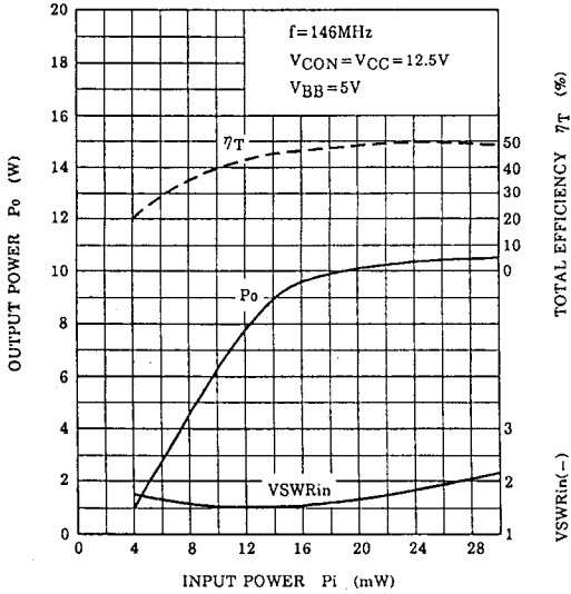
Po, \eta_T , VSWRin - Pi
