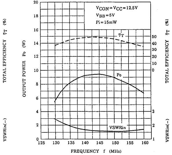
Po, \eta_T , VSWRin - f
